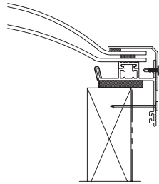
ALB - Aluminum framed skylight with Polyvinyl Chloride (PVC) thermal barrier. Available as curb mounted only. (Shown with optional curb seal tape)
