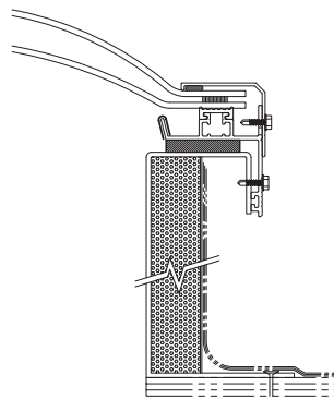
ALIB - Aluminum framed skylight with Polyvinyl Chloride (PVC) thermal barrier and insulated base. Available as self flashing only. (Shown with optional curb seal tape and aluminum double wall)
