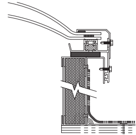
ALT - Thermally broken aluminum framed skylight. Available as curb mounted or self flashing. (Self flashing model shown)
